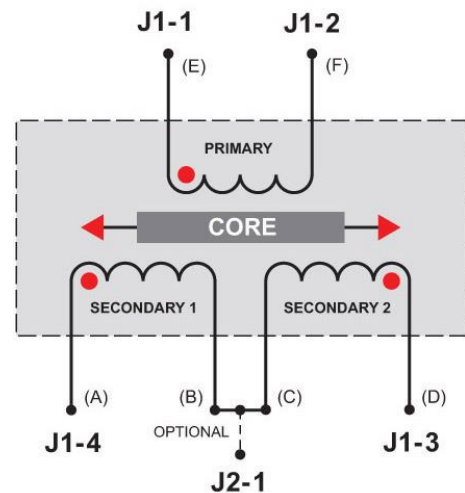
d) 6-Wire LVDTs/RVDTs (see note 5)
